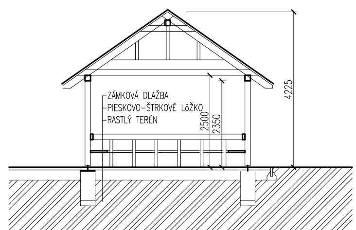
PRIĀĀNY REZ
